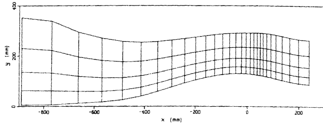
Fig. 5. Stretched grid.
